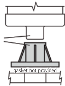
Mounting hole position for pre-drilled adapter (Flange interface to DIN 24557/T2)
