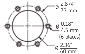
Adapter Part no. VGHD-02081637
