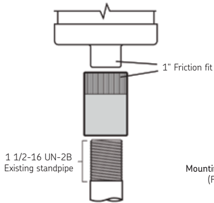
Threaded standpipe adapter Part no. VGHD-02077124
