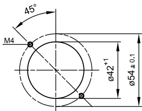
Drilling template for reservoir cover
