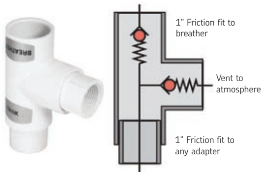
Bypass adapter Part no. VGHD-012708016
